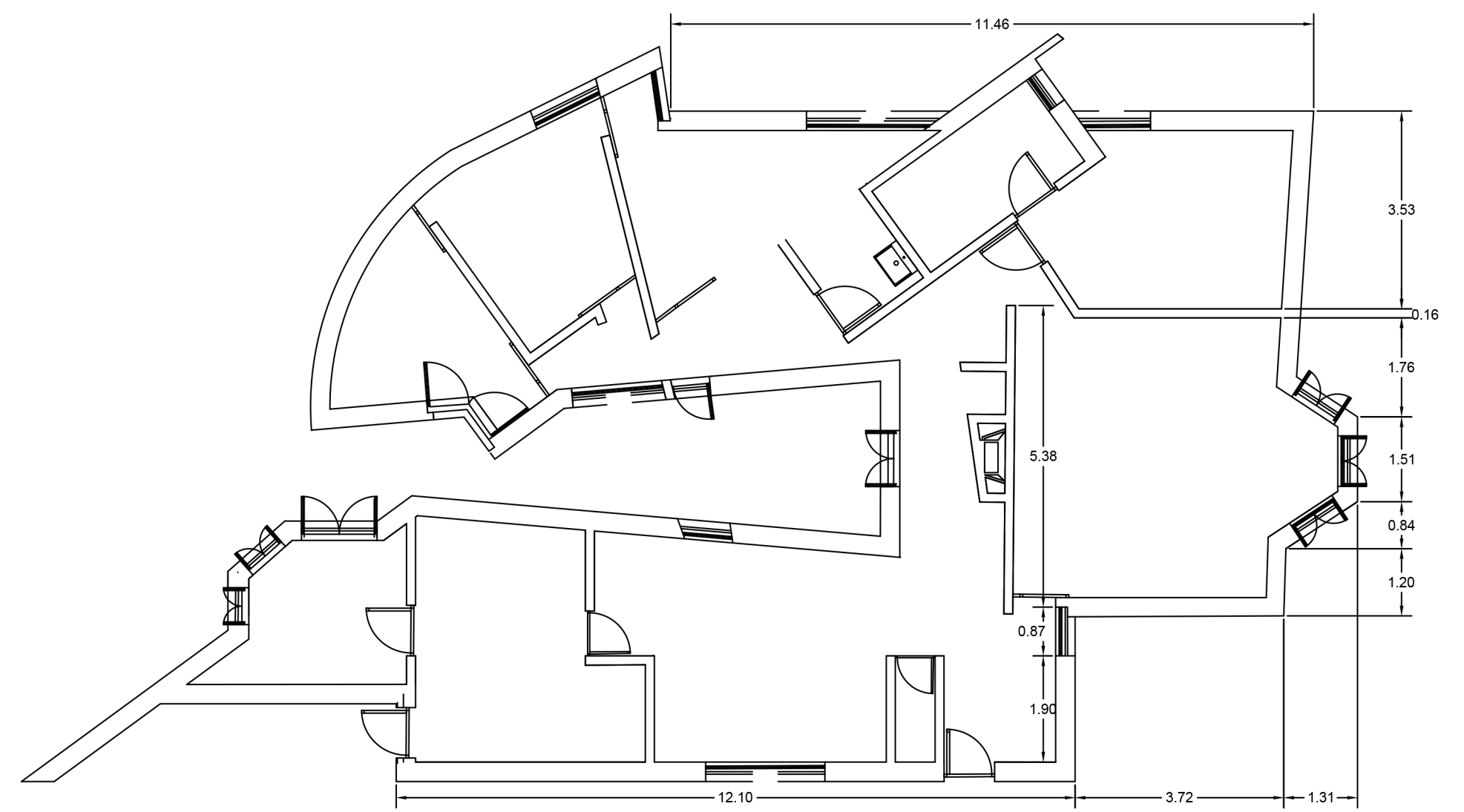
Floor plan 1:100
