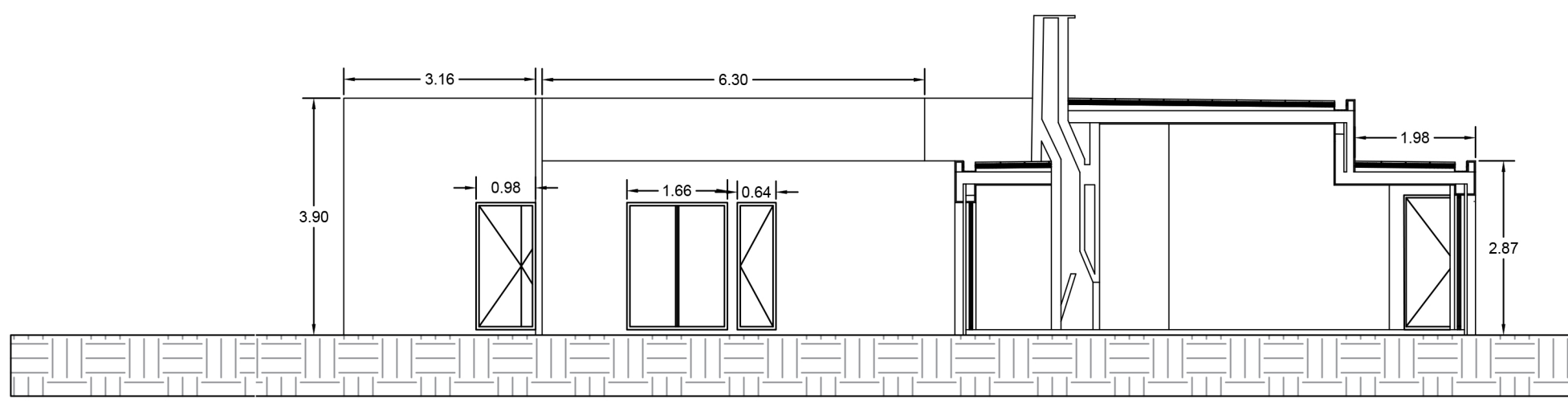
Section 1:100
